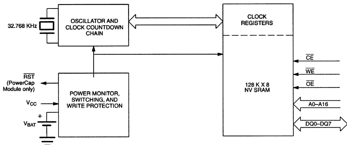
Figure 1. Block Diagram
